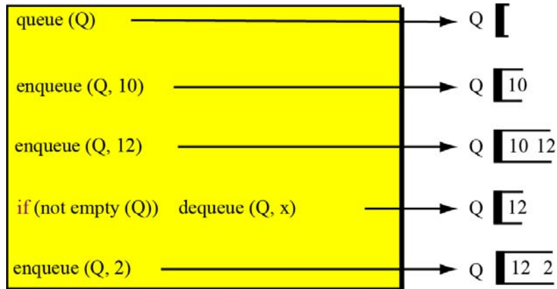
Figure 12.12 Example 12.4
