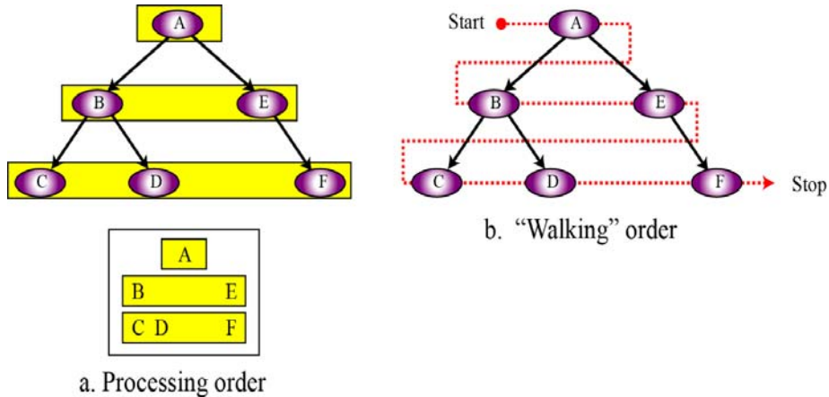
Figure 12.26 Example 12.11
