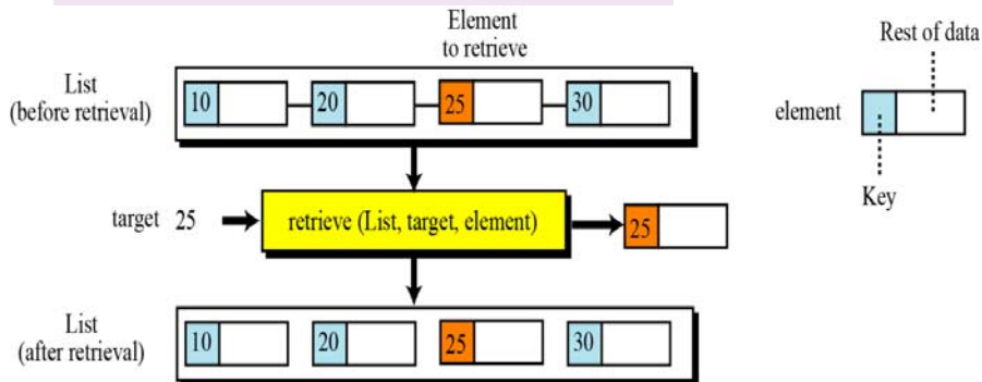
Figure 12.17 The retrieve operation
