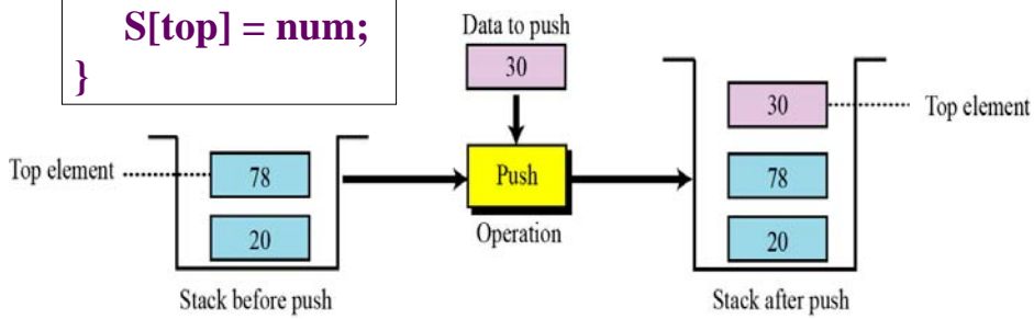
Figure 12.4 Push operation
