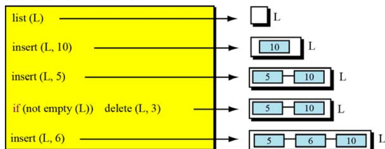
Figure 12.18 Example 12.7
