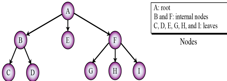
Figure 12.20 Tree representation
