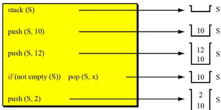
Figure 12.6 Example 12.1
