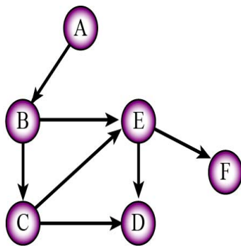
a. Directed graph
