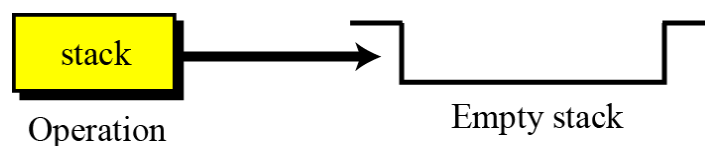
Figure 12.3 Stack operation
