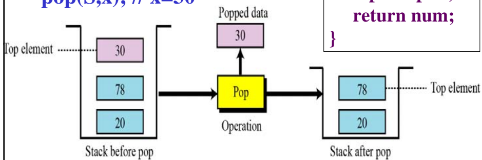
Figure 12.5 Pop operation
