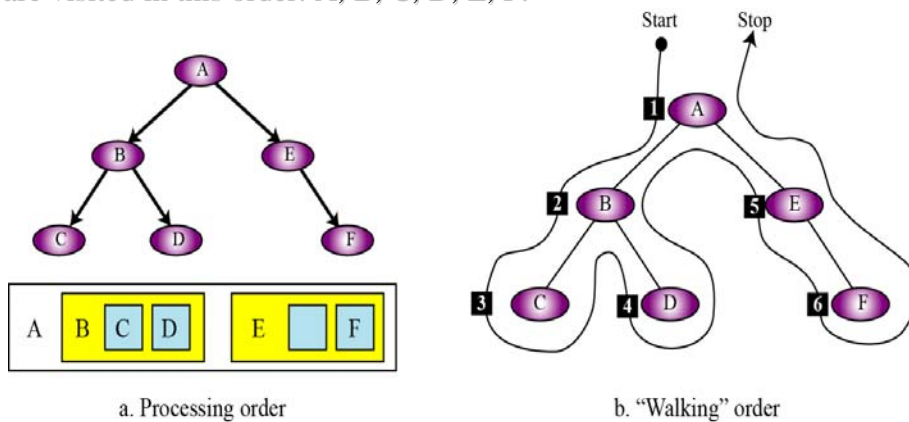
Figure 12.25 Example 12.10
