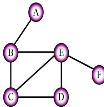
b. Undirected graph
